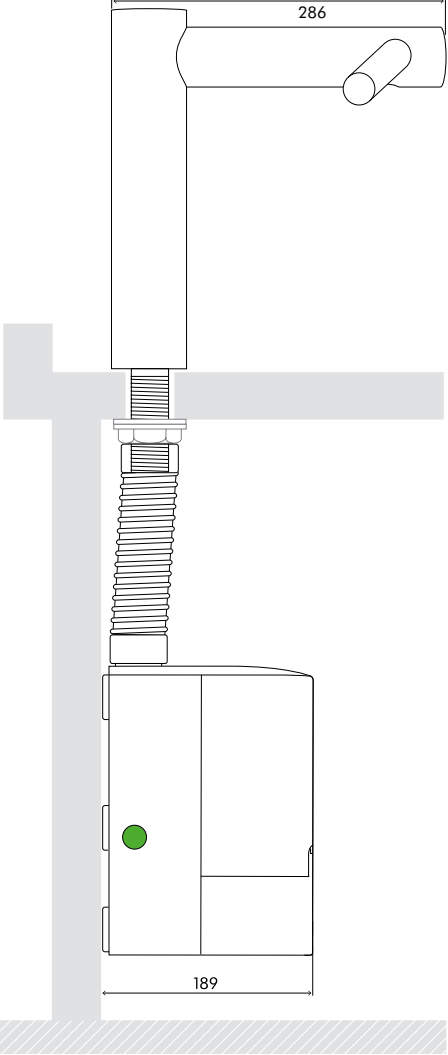
SIDE ELEVATION
